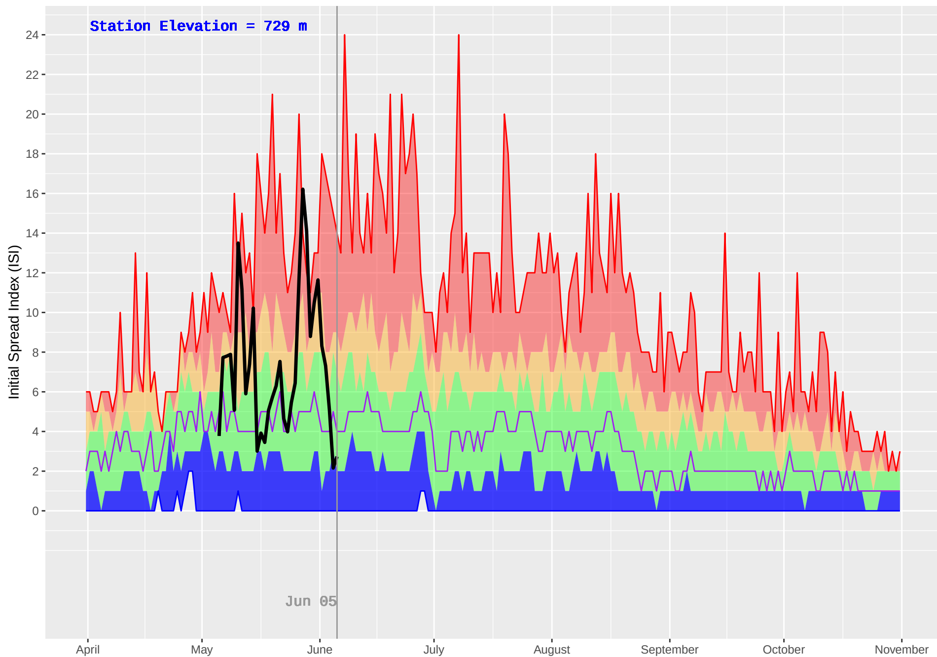
ATLIN (111) : Historical (1977–2018) and Current (2019) Daily Initial Spread Index (ISI)
