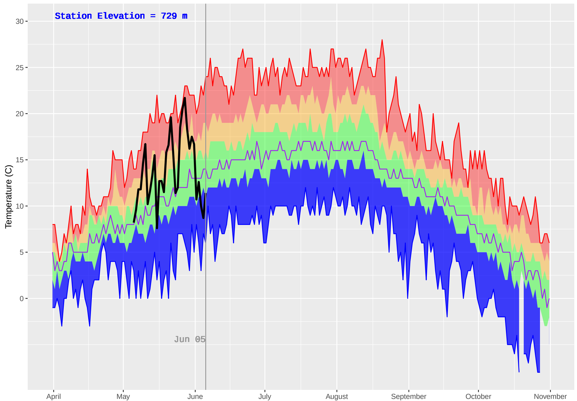
ATLIN (111) : Historical (1977–2018) and Current (2019) Daily Temperature
