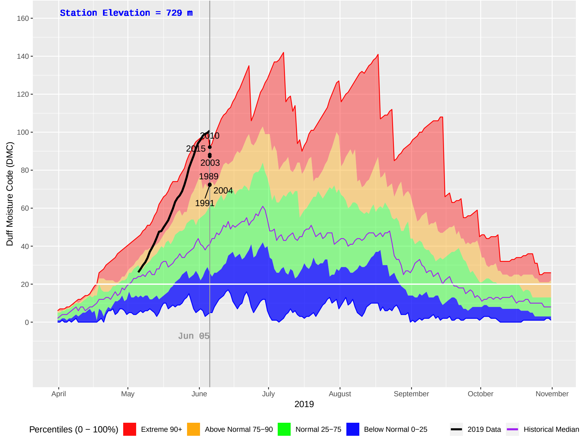
ATLIN (111) : Historical (1977–2018), Current (2019) Daily Duff Moisture Code (DMC)
