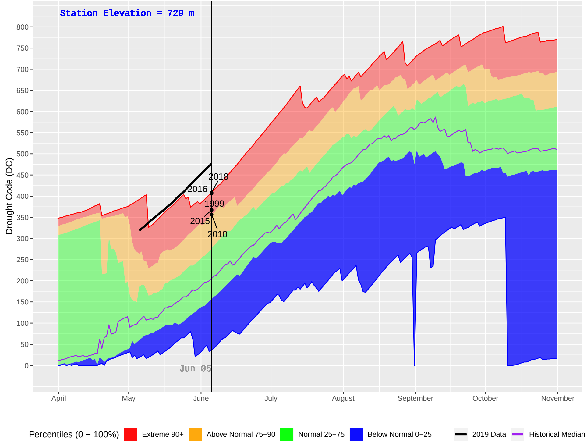
ATLIN (111) : Historical (1977–2018) and Current (2019) Daily Drought Code (DC)
