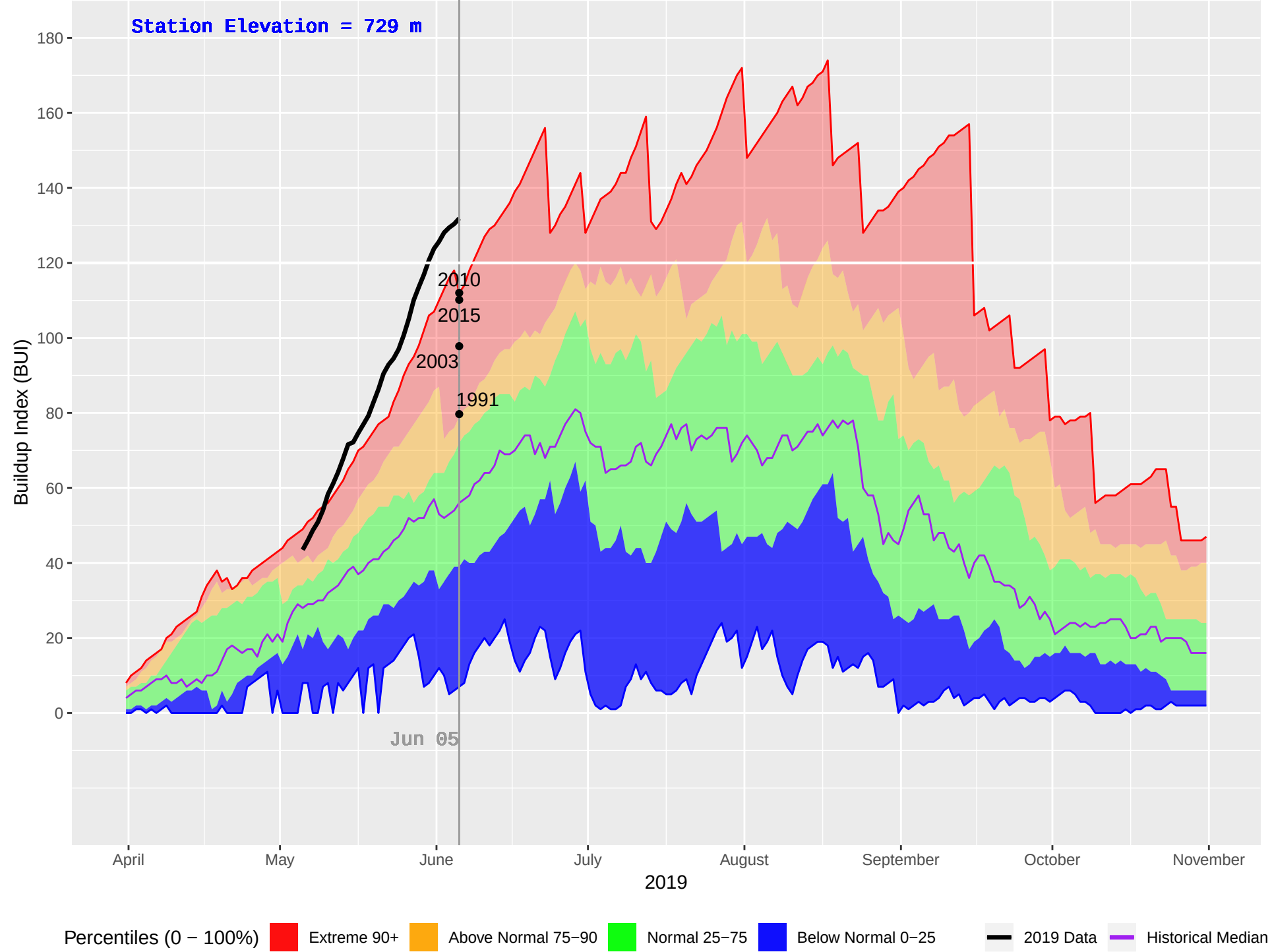
ATLIN (111) : Historical (1977–2018), Current (2019) Daily Buildup Index (BUI)
