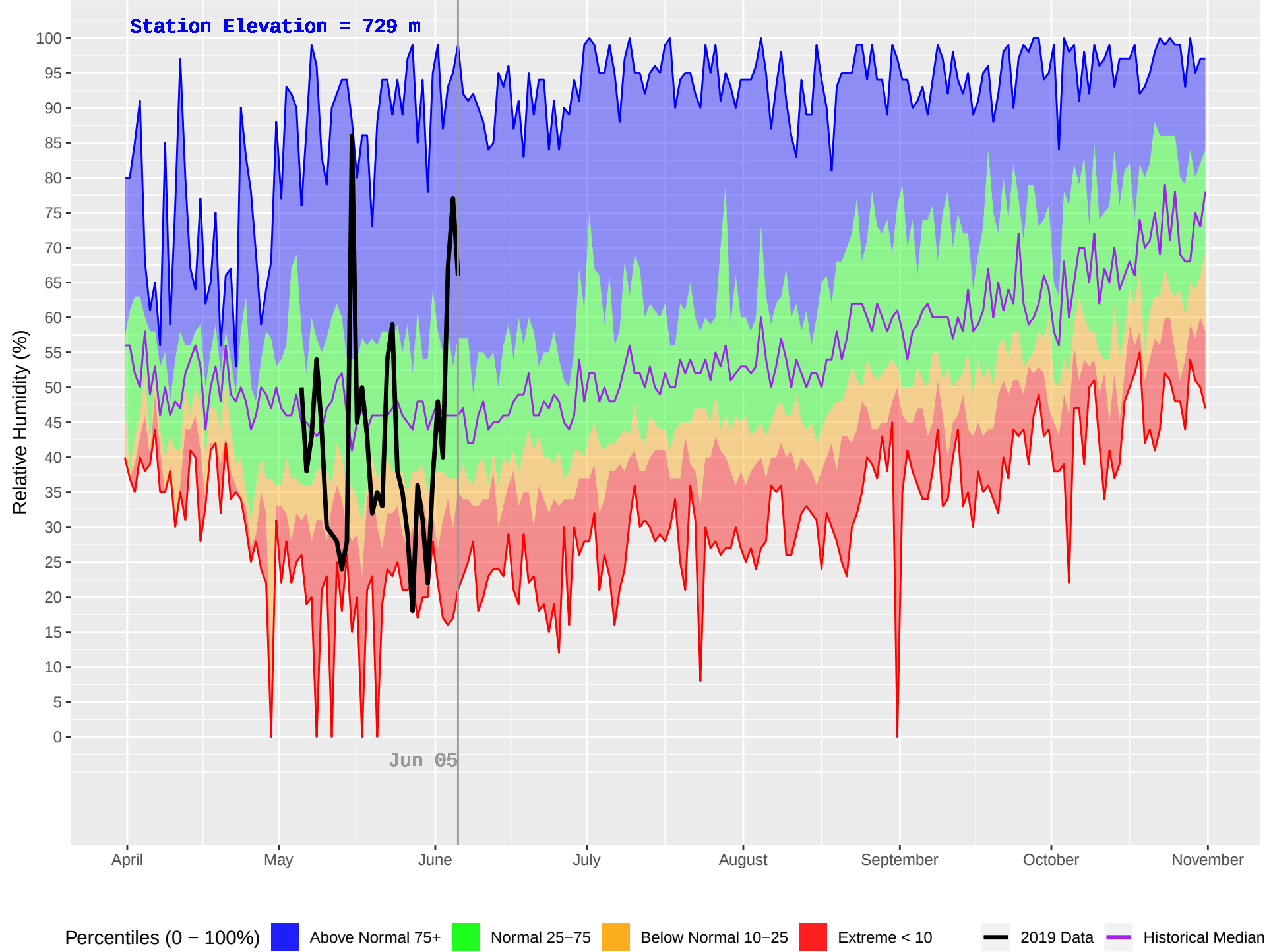
ATLIN (111) : Historical (1977–2018) and Current (2019) Daily Relative Humidity
